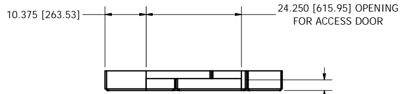
SIDE ELEVATION VIEW
