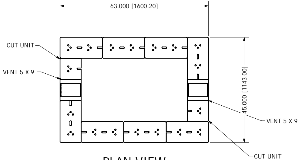
PLAN VIEW
